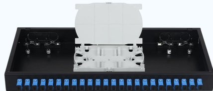
★ 1U 24Core SC/UPC Rack-Mount Fiber Optic Distribution Box
